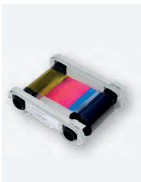
1/3 yellow, pink, cyan blue, 1/3 black and 1/3 overlay ribbon cassette 400 prints per roll.
