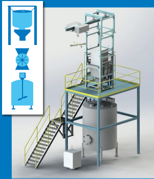
Big bag unloading to conveyor or mixing
